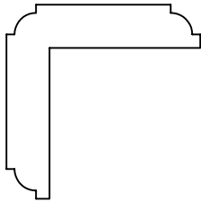
WM 202 KN#'s 48 & 49 WOOD SIZE: 1\frac{1}{8} " x 1\frac{1}{8} "
